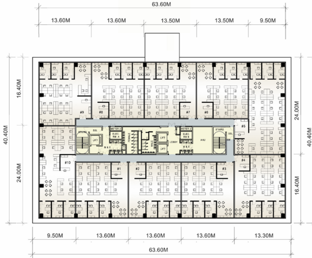
1st to 4th Floor Plan
